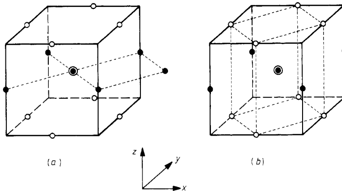
Figure 4. FCC structure built up by manganese ions of one magnetic sublattice (central ion and 12 neighbours). Ions marked by \bullet and \circ , respectively, are equivalent considering the {}^4T_{1g} substate. (a) Simple quadratic lattice formed by equivalent manganese ions of one xy plane. (b) BCC structure consisting of the central ion and its eight equivalent neighbours.
